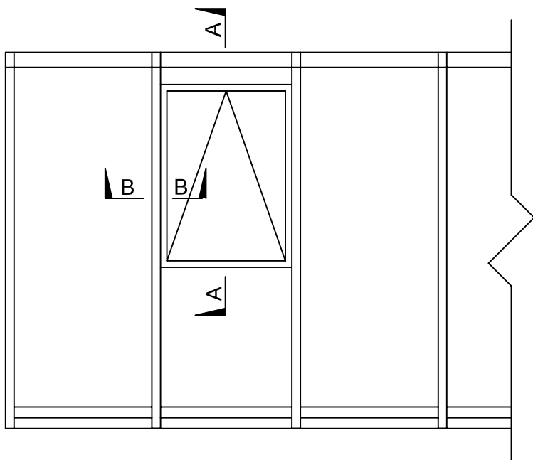
Typical Elevation
